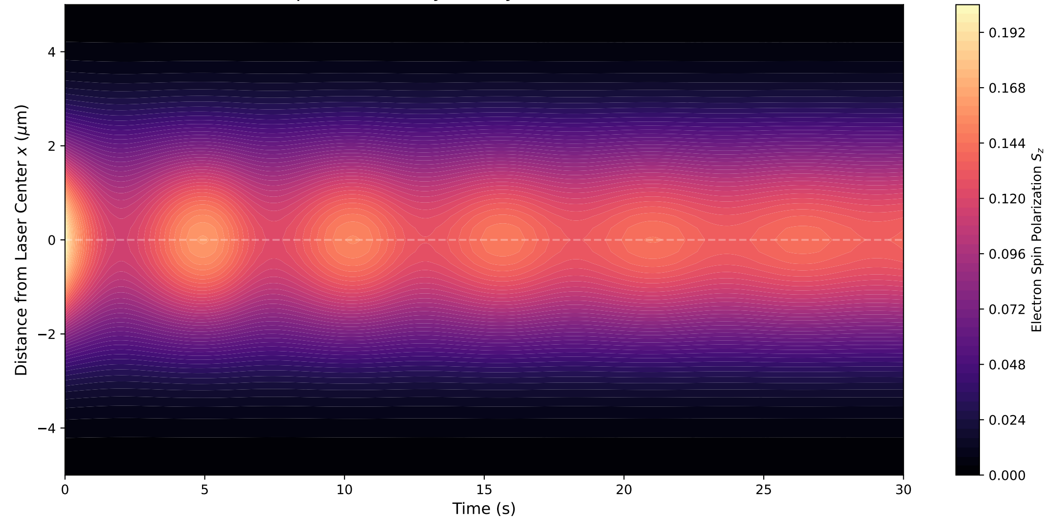
1D Spatial Time Crystal: Synchronization Waves
